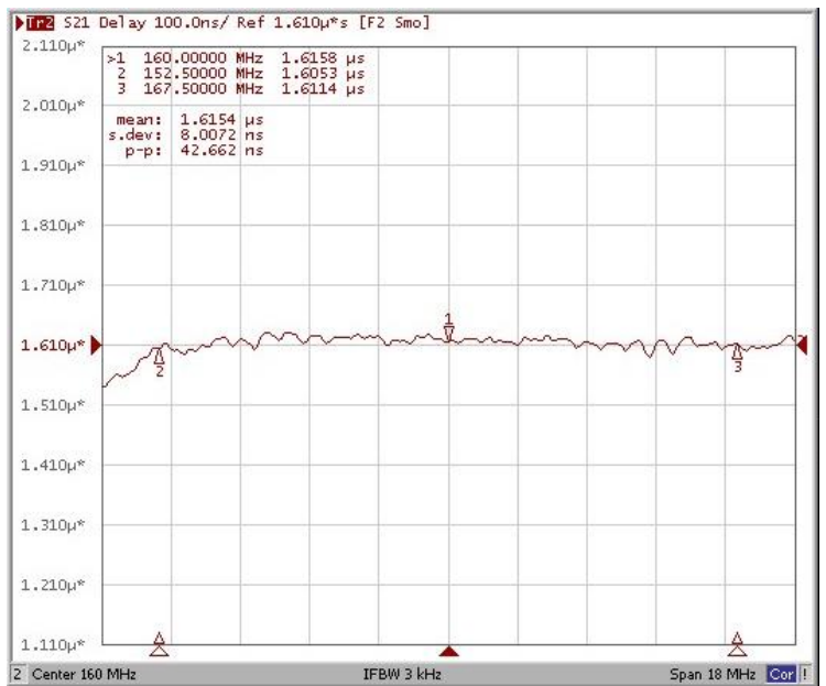
Group Delay Variation Fo \pm 7.50 MHz
