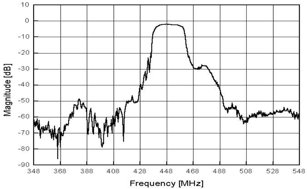
Frequency Response
