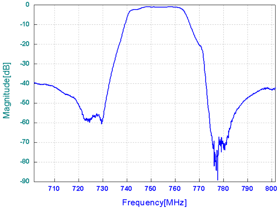
Frequency Response
