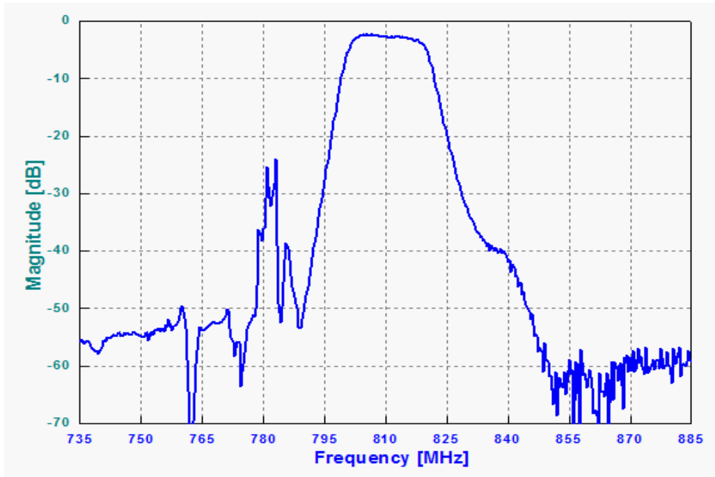
Frequency Response
