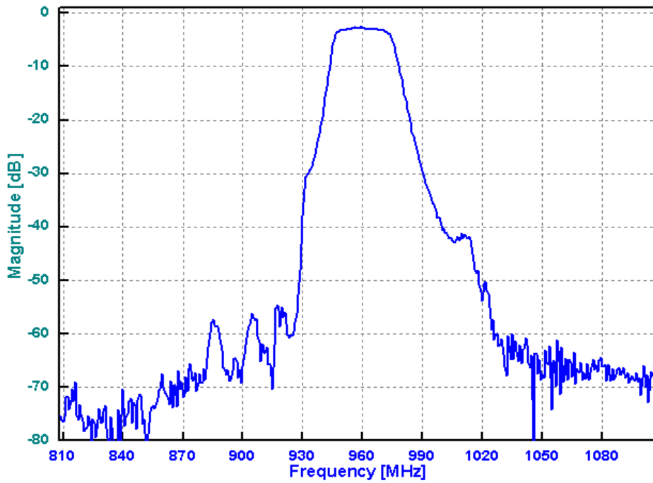
Frequency Response
