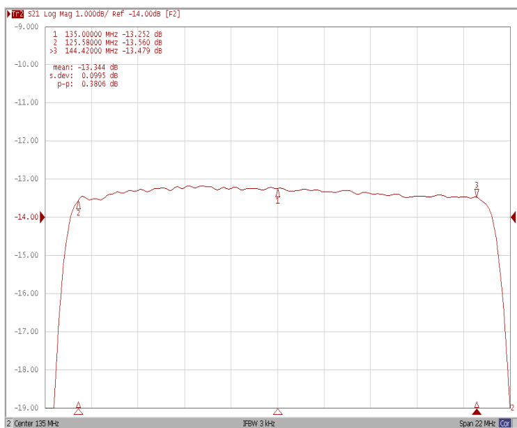
Ripple Variation Fo±9.42MHz
